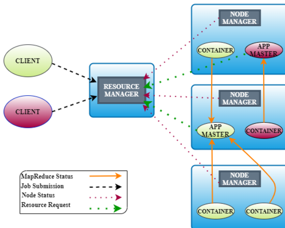
Figure 2.1.3.1: YARN Architecture
