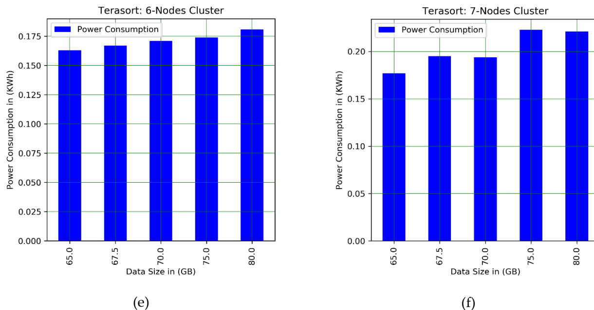
Figure 5.1.1.1: Power Consumption vs Terasort Workloads on Hadoop Cluster
