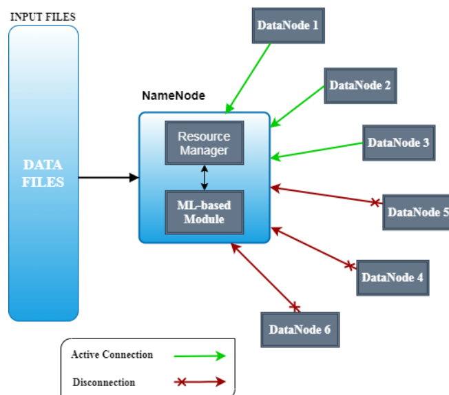
Figure 6.4.3: Example of Decommissioning 3 DataNodes based on the ML-based Module
